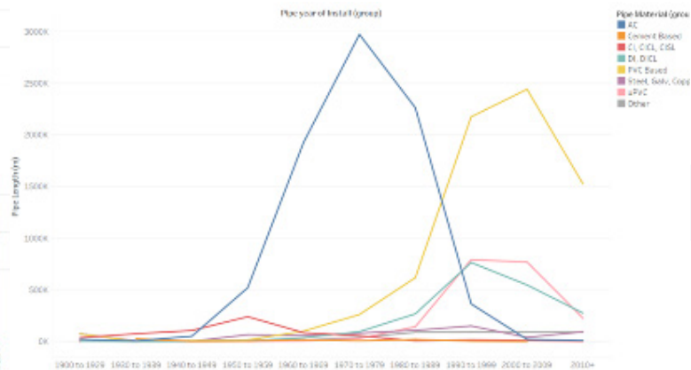
Installation of water pipes installed by 27 service providers
